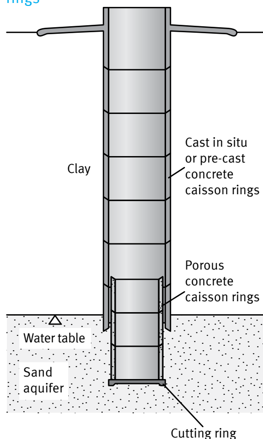
Fig 4: Example of excavation below water table using concrete caisson rings
