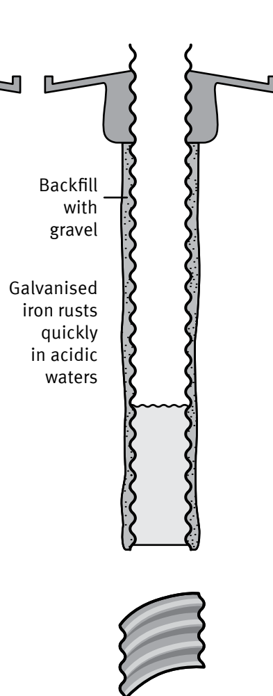
Each circle of galvanised iron is composed of three curved sections bolted together
